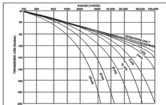
Figure 2-23. Spherical Spreading and Absorption Loss as Related to Frequency and Range
